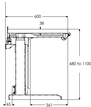
Freestanding Table Side Elevation
