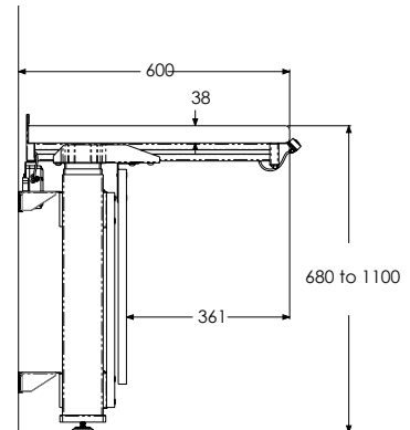
Wall Mounted Table Side Elevation
